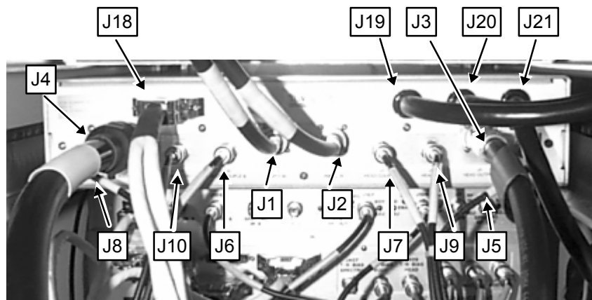
RFI MODULE REAR CONNECTIONS ILLUSTRATION 4-2
